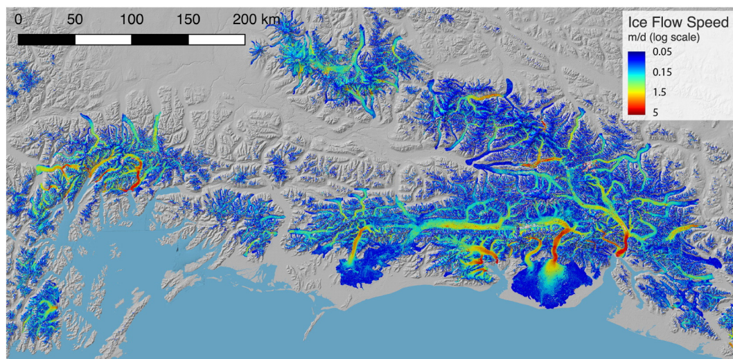
Fig. 11. Mosaic of ice flow speed for the glaciers of southern Alaska, from College Fjord and Columbia Glacier in the west to the Alek River in the east, with Wrangell-St. Elias in the mid-upper part of the map. This mosaic, posted at 200 m, is composed of trackable Landsat 8 pairs from 2013 to 2015. The coverage is sufficiently sampled in time to develop quarterly (90-day) maps of ice flow speed over the Landsat 8 record for most areas. Base image is a shaded relief from Kienholz, Rich, Arendt, & Hock, 2014; image-pair offset correction used a land mask from Kienholz et al., 2015.
