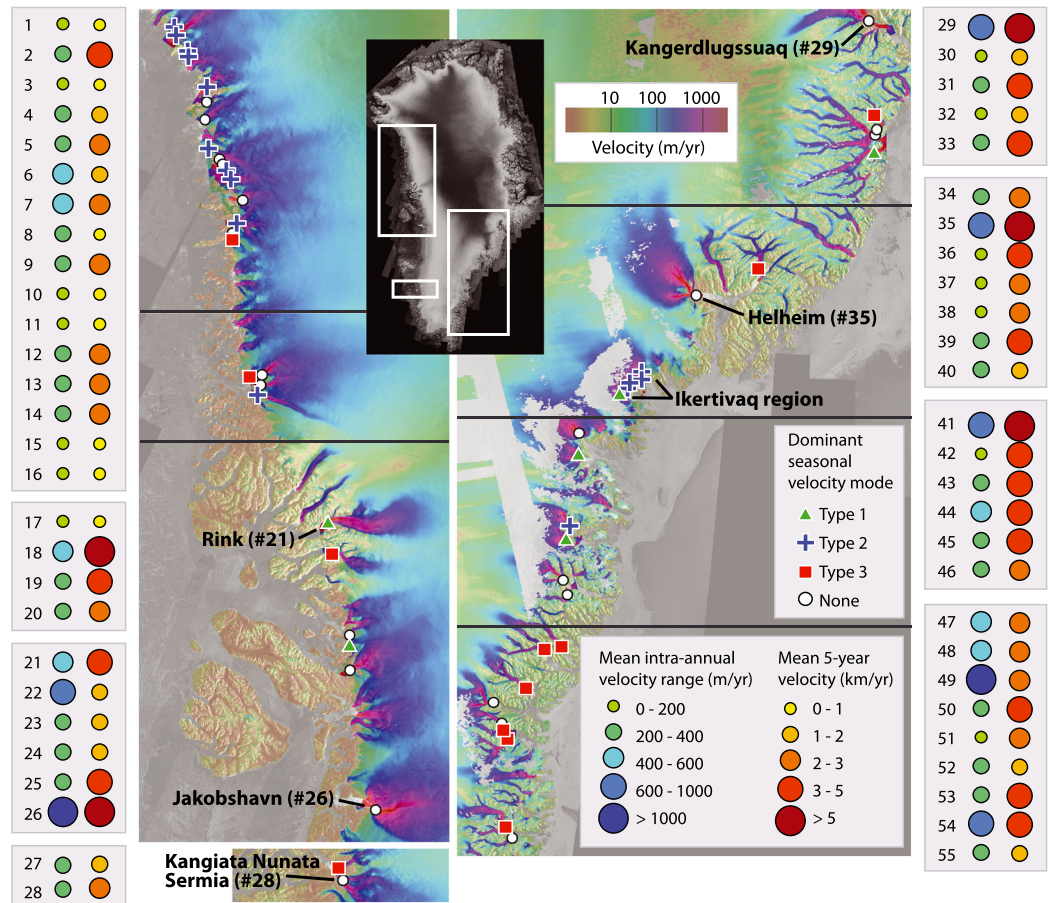
Figure 1. Mean intra-annual velocity range, 5 year mean velocity, and seasonal velocity mode for Greenland marine-terminating outlet glaciers. Center panels show the locations for the 55 study glaciers, with symbols indicating the dominant seasonal velocity mode. Background map shows RADARSAT mosaic of surface velocity. Side panels indicate the mean intra-annual velocity range (m/yr, blue-tone circles) and mean 5 year velocity (km/yr, red-tone circles) for each glacier (identified numerically) in north-to-south order corresponding to glaciers in center panels (divided into segments for easier reference).
