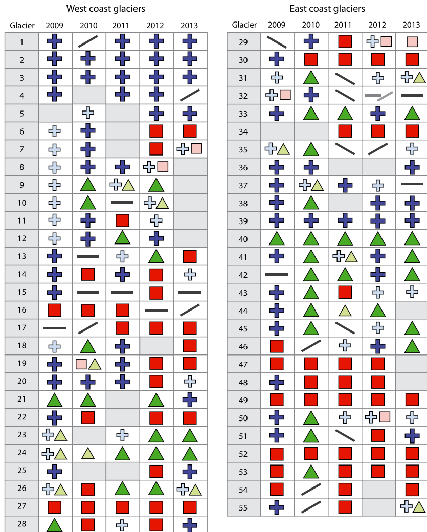
Figure 3. Seasonal velocity modes for Greenland outlet glaciers by year. Symbols designate the seasonal velocity pattern for each glacier for every year (triangle = type 1; cross = type 2; square = type 3), with straight lines indicating consistently accelerating, decelerating, or flat speeds (<50 m/yr range) during the year. Lighter, smaller symbols indicate that the designation is based on limited data or has components of two patterns. Lighter, smaller crosses (blue) may also indicate that there was a summer spike but a higher measured velocity in winter or late fall. Gray boxes indicate insufficient data for identifying patterns. (See Figures S1–S55 for velocity data for individual glaciers).
