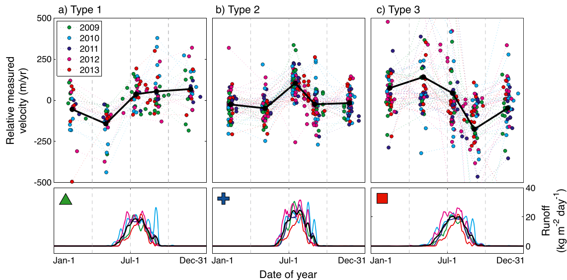
Figure 2. Marine-terminating Greenland outlet glaciers with distinct seasonal velocity modes and associated ice sheet runoff. Top row: Plots include all glaciers with dominant seasonal velocity modes for (a) type 1, (b) type 2, and (c) type 3 behavior (as shown in Figure 1 and discussed in text). Mean velocity pattern is indicated (thick black line). Bottom row: Smoothed daily runoff ( \text{kg}/\text{m}^2/\text{d} ) from RACMO2.3 for 2009–2013 for glaciers with the designated dominant seasonal velocity mode. Mean runoff is included for each year (colored lines) as well as the 4 year mean runoff (black line).
